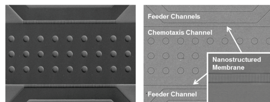
Figure 1. (A) A silicon and polymer master is formed using a combination of electron beam lithography, anisotropic silicon etching and crosslinkable polymer. (B) This master can be replicated in silicone to form a microfluidic chamber with nanostructured membranes that allow material exchange during real-time imaging of the microbial response
