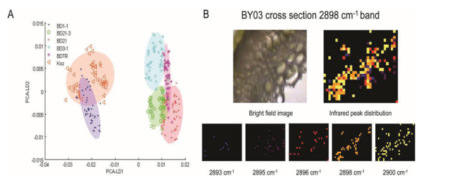
Figure 2. Chemical analysis of Brachypodium samples using mid-IR. (A). The PCA-LDA score plot of samples from 6 Brachypodium lines. 45 spectra are collected from each line. Spectra data are collected from 600 \text{cm}^{-1} to 4000 \text{cm}^{-1} . The spectra in the region between 800 \text{cm}^{-1} and 1200 \text{cm}^{-1} are used as input for PCA-LDA analysis. The “Bd1-1” and “Koz-3” samples are clearly separated from the other 4 types of samples. (B). The distribution and shift of the 2898 \text{cm}^{-1} band in the cross section of a Brachypodium sample thin slice. Each peak position is represented by a different color.
