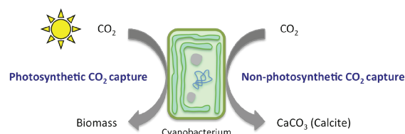
Figure 1. Two modes of CO 2 uptake in cyanobacteria.
