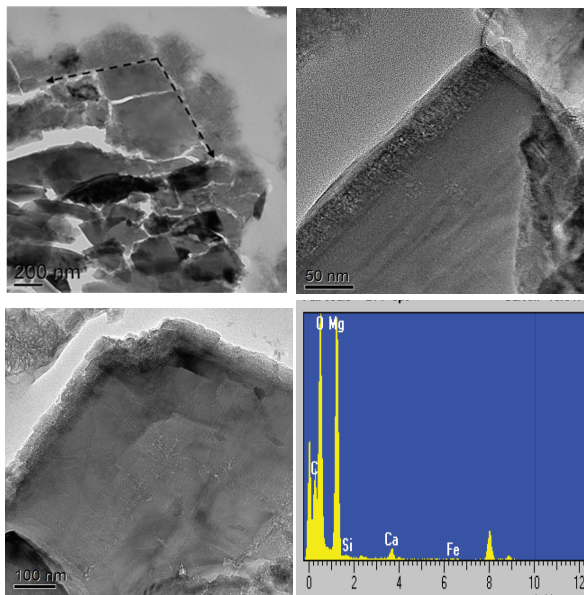
Figure 2. Crystallites from upper layer of the Hot Lake mat sampled just above the green cyanobacterial layer. The crystallites are magnesite ( \text{MgCO}_3 ) as determined by selected area electron diffraction (SAED) with amorphous coatings of similar elemental composition as determined by energy dispersive X-ray spectroscopy (EDS).
