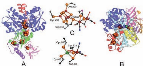
Figure. Structures of (A) Cpl H_2 ase, (B) [NiFe] H_2 ase, (C) H-cluster, and (D) NiFe active site.
