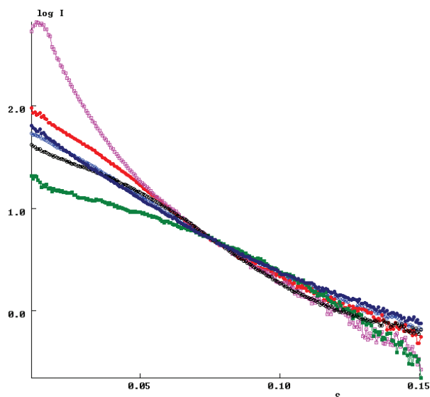
Figure 1. SAXS experiments on ParA, ParB, and parS demonstrate oligomerization upon addition of ATP (purple curve) compared with the sample without ATP (red curve). We thank Greg Hura of the ALS SIBYLS beamline 12.3.1 for assistance with the SAXS experiments.
