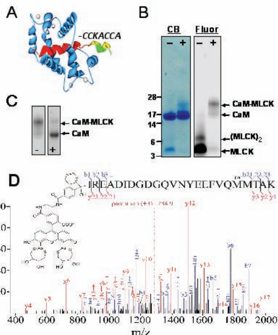
Figure 2: Mass Spectrometric Identification of Interfacial Binding Site Following Crosslinking and Fluorophore Transfer. (A) Depiction of the structural interface between tagged MLCK protein (red) containing engineered TRAP binding site CCKACCA (yellow and green) in complex with binding partner CaM (blue). (B) Coomassie Blue (CB) protein stain and fluorescence from TRAP reagent (Fluor) prior to (-) and following (+) photo-induced crosslinking. (C) Cross-linked complex before (-) and following (+) transfer of TRAP to binding partner upon addition of DTT (5 mM). (D) Mass spectrum of TRAP-bound peptide, where all b (blue) and y (red) fragment ions are identified. Site of TRAP binding in CaM bait protein is shown above mass spectrum.
