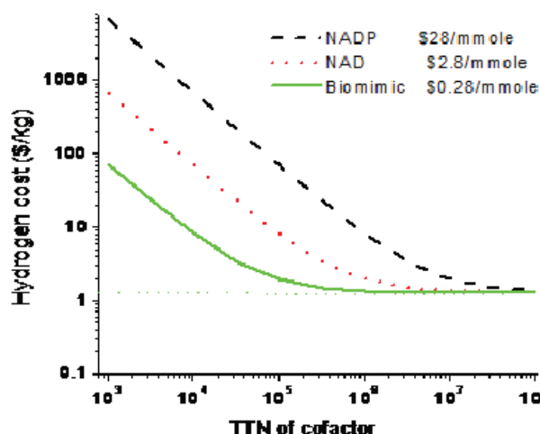
Fig. 4. The estimated hydrogen production costs in terms of turnover number of enzymes and co-enzymes. Carbohydrate prices are $0.18 per kg [2].
