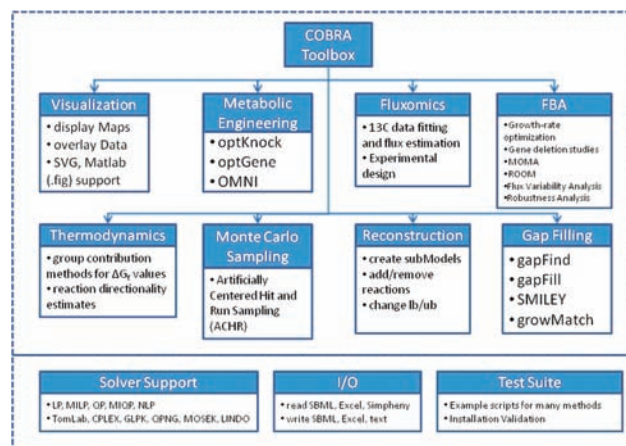
Figure 1: Features of the COBRA toolbox: Top) Scripts are available for methods in eight areas of metabolic systems biology. Bottom) Linear and Quadratic solvers are implemented through a simple yet flexible API in a vendor independent fashion. A set of test scripts are present to validate proper installation as well as demonstrate examples of use.
