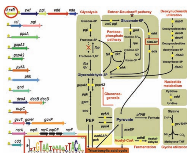
Fig. 1. The reconstructed HexR regulon and target pathways in Shewanella oneidensis MR-1.
