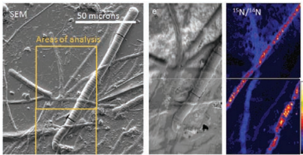
Fig. 1. Scanning electron microscopy (SEM) micrograph and NanoSIMS secondary electron (e-) and nitrogen isotope ratio ( ^{15}\text{N}/^{14}\text{N} ) tiled images of the cyanobacterial community of the Elkhorn Slough microbial mat. The mat was incubated in ^{15}\text{N}_2 for 9 hours during the night prior to sampling. Cyanobacteria that were fixing nitrogen incorporated the ^{15}\text{N} tracer. The color scale bar represents ^{15}\text{N}/^{14}\text{N} ratios of 0.003 (black) to 0.09 (white).
