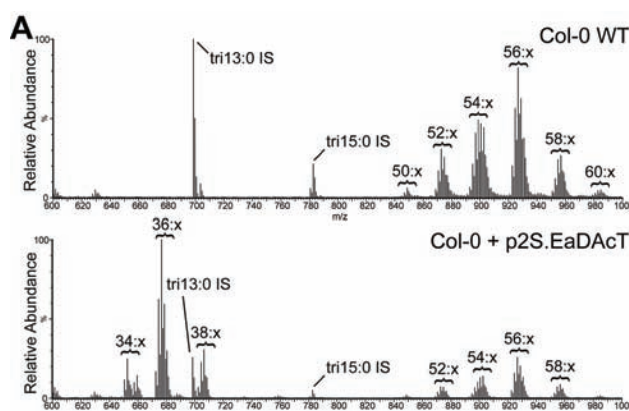
Fig 2. Arabidopsis seeds expressing EaDacT accumulate ac-TAGs. Positive-ion ESI mass spectra of neutral lipid extracts from Col-0 wildtype seed or T 3 seed from a representative Col-0 plant expressing EaDacT. Peaks correspond to m/z values of the [M + NH 4 ] + adduct. Tridecanoin (tri13:0) and tripentadecanoin (tri15:0) were added as internal standards. The number of acyl carbons in each series of TAG molecules is indicated.
