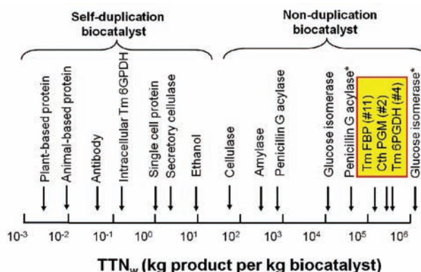
Fig. 3. Comparison of weight-based total turn-over number (TTNw) of self-duplication living biocatalysts and non-duplication enzymes [1, 3].
