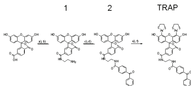
Scheme 1. Synthesis of TRAP. A) EDC, Et 3 N, NHS, dry DMF, 30 min; B) N -Boc-ethylenediamine, 16 h; C) 20 % TFA/CH 2 Cl 2 , 2 h; D) 4-Benzoylbenzoic acid, EDC, NHS, iPr 2 EtN, DMF, 16 h; E) HgO, TFA, 70 °C; F) 1) AsCl 3 , PdOAc, iPr 2 EtN, NMP, 4 h; 2) EDT, 20 % acetone/H 2 O (overall yield: 2 %).
