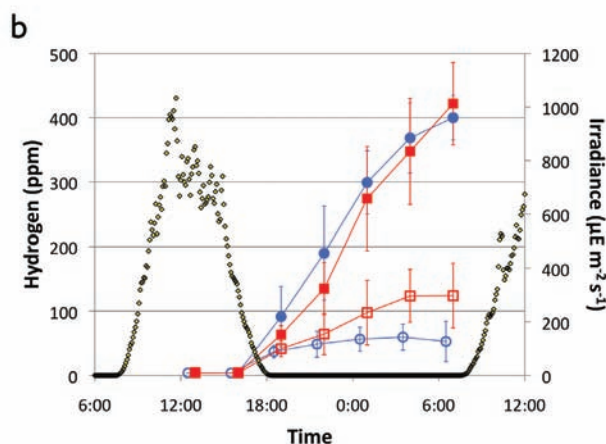
Fig. 1. Net hydrogen production in Elkhorn Slough microbial mats. (a) Effect of photoperiod deprivation (red filled diamonds), 20 \mu M DCMU (red unfilled diamonds), 30 mM molybdate (filled blue circles) and homogenization (green filled triangles) compared to a control (unfilled blue circles) on H 2 production. (b) Effect of N 2 -fixation suppression on H 2 production under control and SRB inhibited conditions. 8.8 mM ammonium added to suppress N 2 -fixation (red squares) and compared to N 2 -fixing incubations (blue circles). Filled red squares and filled blue circles signify incubations with 30 mM molybdate.
