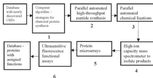
Figure 1. Modular high-throughput platform for fast and parallel total chemical synthesis, mass-spectrometric purification and single-molecule spectroscopic assay to annotate function for newly predicted proteins.
