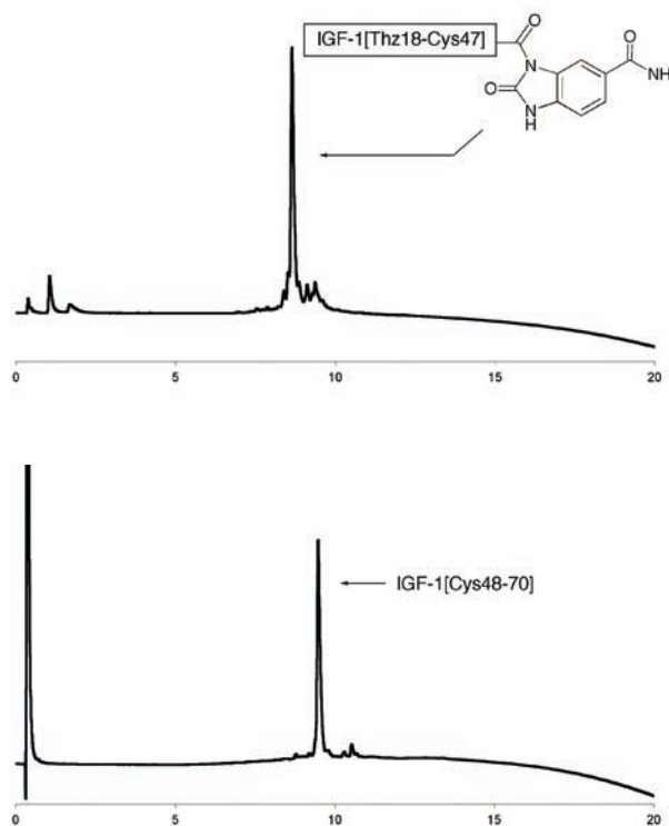
Figure 2. Automated robotic Fmoc SPPS preparation of peptide-thioesters. HPLC-electrospray MS of crude products are shown.
