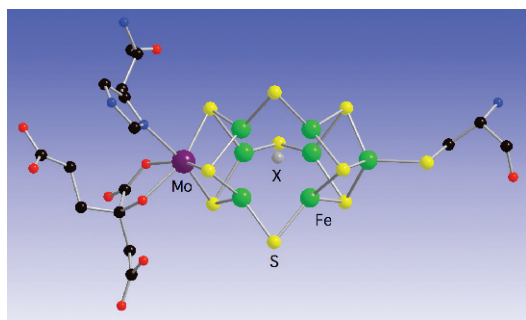
Figure. Structure of the nitrogenase FeMo-cofactor.
