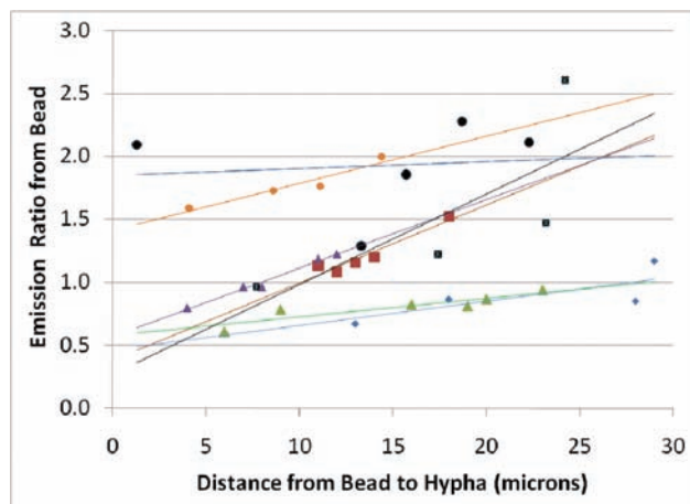
Figure 1: Fluorescent emission from individual beads as a function of distance from hypha. Lower Y axis values indicate more oxidation.
