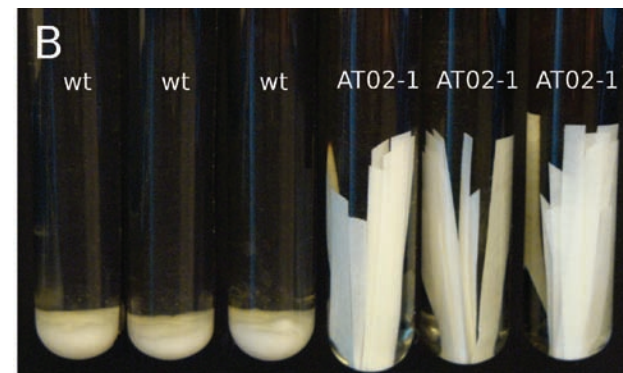
FIG 1 C. phytofermentans strain with disruption of cphy3367 (AT02-1) had similar growth rates as wild-type on glucose A, but had lost the ability to degrade filter paper cellulose B. Growth curves are means of triplicate cultures. Error bars show one standard deviation and are smaller than the symbols where not apparent.
