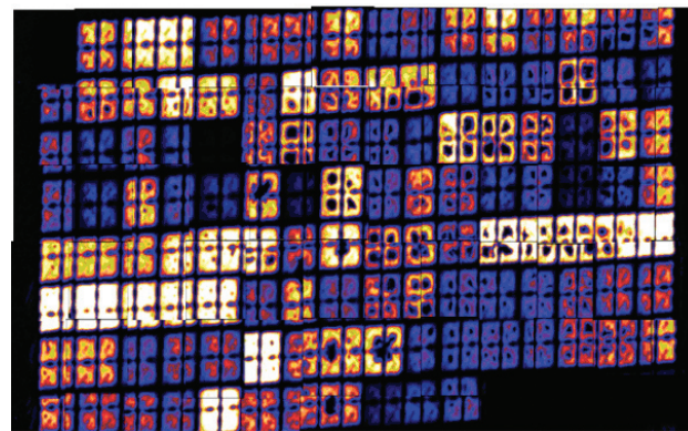
^{13}\text{C} enrichment by nanoSIMS
