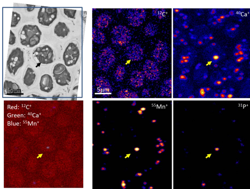
Fig. 1. Correlated STEM and NanoSIMS ion images. The location of the cells can be visualized in the C and Ca ion images. The color addition image (lower left) combines the NanoSIMS \text{C}^+ , \text{Ca}^+ and \text{Mn}^+ images. The arrows indicate the same location in all images. Inspection shows that Mn foci tend to correlate with Ca and P foci. Count rates for P are relatively low because of low \text{P}^+ yield.
