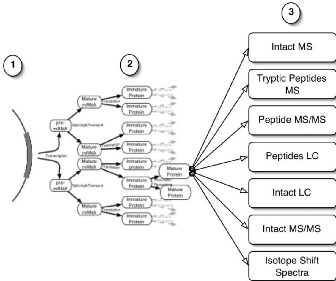
Figure 1. The three primary components of the PIE. 1) The identification (inward) step locates putative genomic origin(s) for the sample. 2) The outward projection step predicts putative mature protein products that might originate from the locus found in step 1 using a breadth-first, heuristically-bounded search. 3) Each putative product is mapped through plug-in modules representing the separation and detection methods used, with Bayes statistics used to assign a probability score for the putative product based upon how well the artificial spectra match the details of the real spectra.
