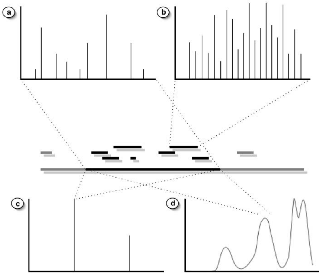
Figure 2. The outward-projection from a genomic region to mass spec data. The putative protein products of this sequence region can be matched against a variety of data collected in the laboratory, including a) peptide mass fingerprint, b) tandem mass spectra, c) intact mass measurements, d) LC profiles (UV).
